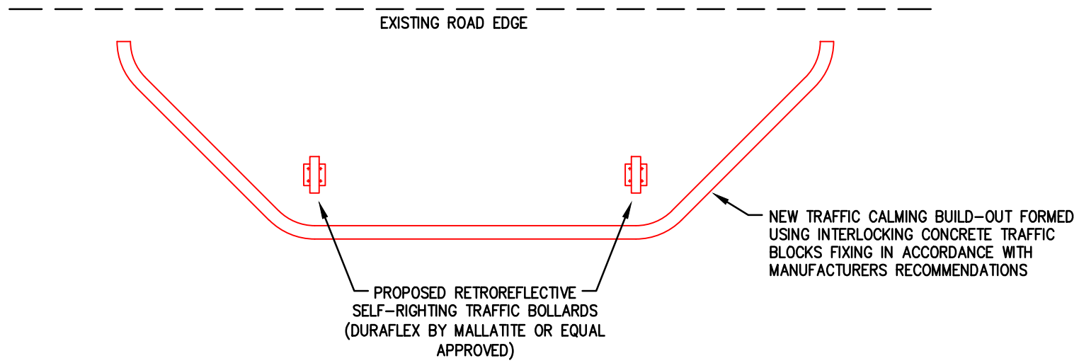
TYPICAL TRAFFIC CALMING BUILD-OUT LAYOUT 1:50
